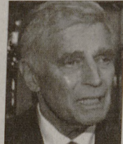
HESTON
