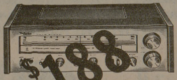
KENWOOD SA-200 FM/AM stereo receiver. 25 watts per channel, minimum RMS into 8 ohms, from 20-20,000 Hz, with no more than 0.04% total harmonic distortion. $188
