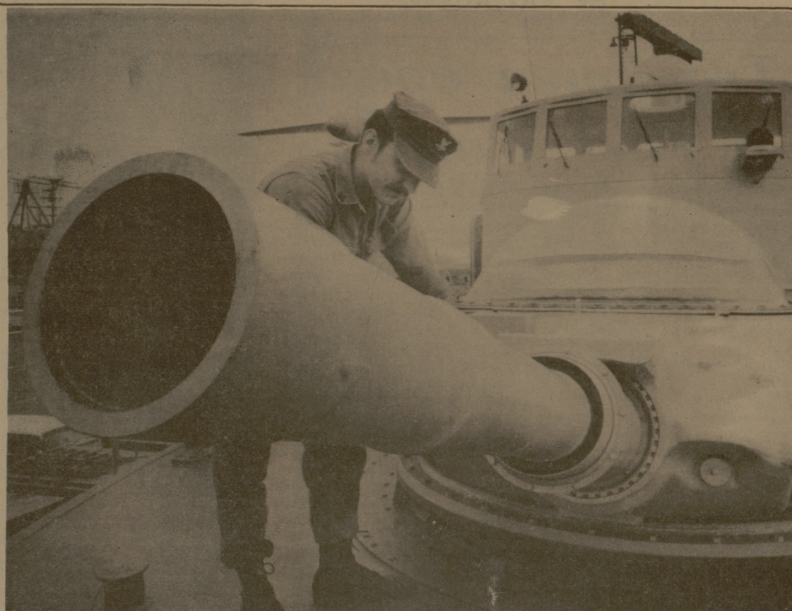
CHECKING OUT THE MUZZLE of a 6-inch tank gun mounted on the Navy's hydrofoil warboat Flagstaff is Gunner's Mate 2.C William Thomas. Thomas went to Army school to learn its operation, just like those on the giant Sheridan tanks.
