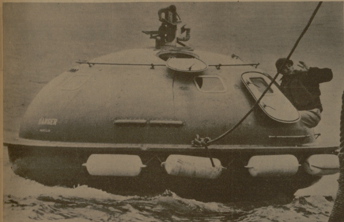
A COAST GUARDSMAN sits in the hatch of a glass fiber sphere, known as the Brucker survival capsule, as it was tested in New York harbor for lifeboat purposes. Weighing five thousand pounds and 14 feet in diameter the unusually shaped life boat is for use in emergency situations at sea. Preliminary testing has been promising. (AP Wire-photo)
