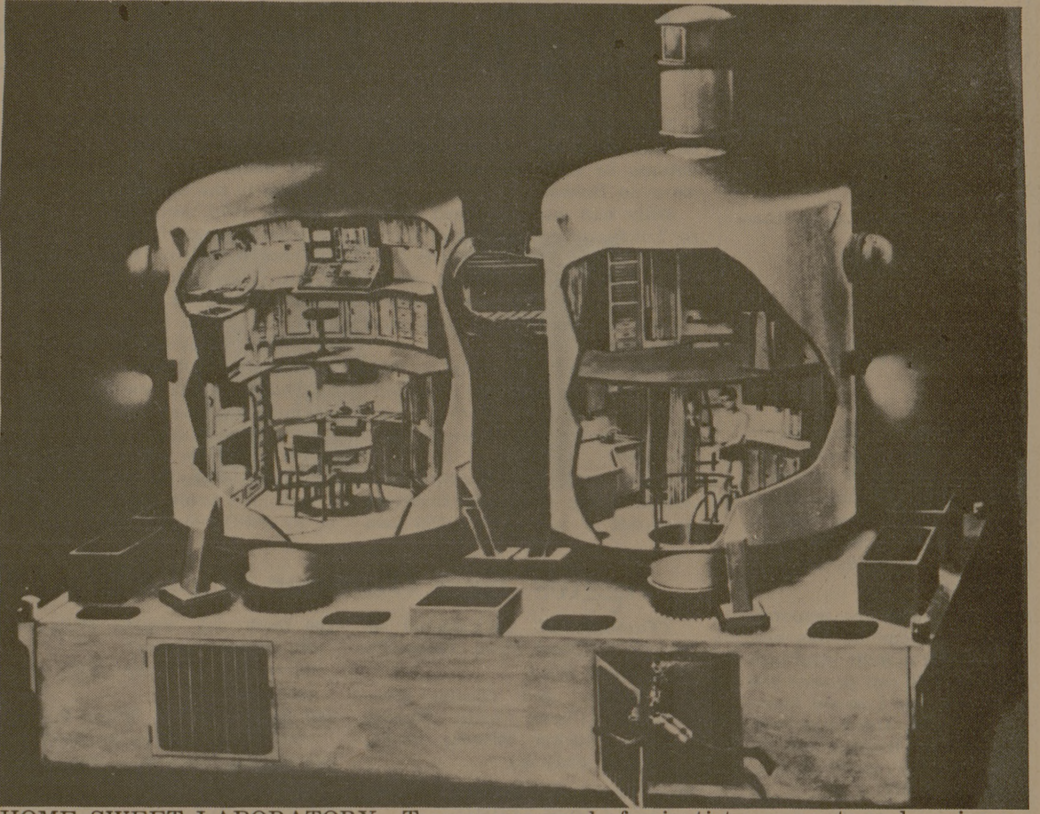
HOME SWEET LABORATORY—Teams composed of scientist-aquanauts and engineers will call this four-chamber, General Electric-built habitat home for periods ranging from 14 to 30 days.
