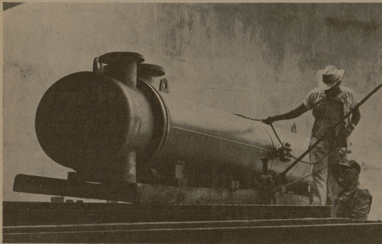
FIVE-TON MOVING JOB Workmen skidded, jacked and levered a five-ton, 20-foot long nuclear reactor heat exchanger through a hole in the wall into position at the Nuclear Science Center Wednesday. The apparatus is part of the cooling installation for a ten-fold reactor power increase, to one megawatt, early in 1968.
