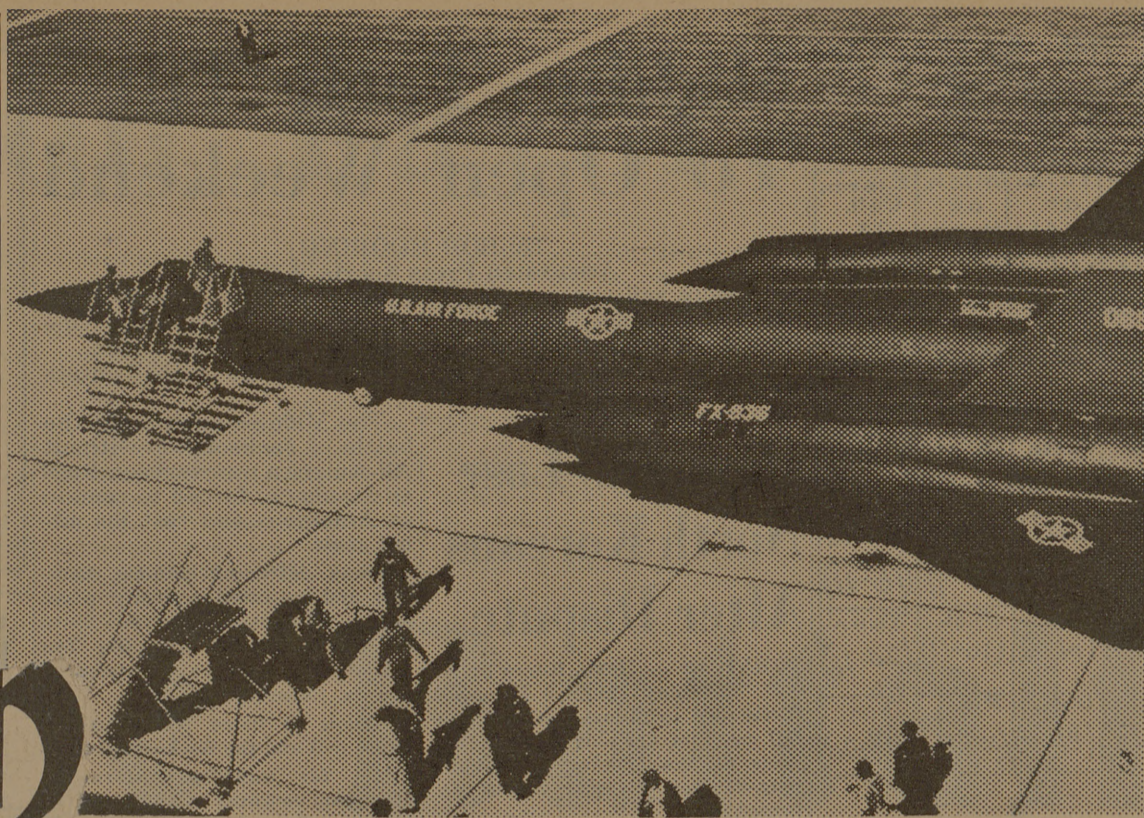
Secret Interceptor top secret YF12A interceptor, capable of flying three times the speed of sound (2000 m.p.h.), stands on a ramp at Edwards Air Force Base, Calif., in its first public appearance.
