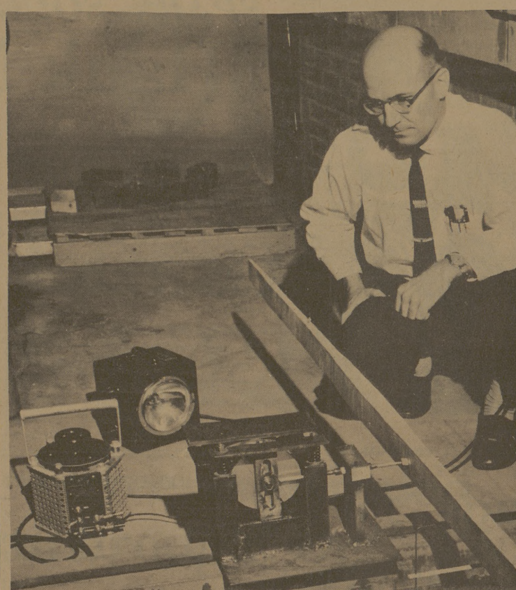
ME Prof With Project Professor T. A. Noyes poses with a setup he and students built for class use in ME Course 459 to attempt to simulate lateral vibrations of X-15 aircraft during flight. A research project is expected to be established along similar lines with sponsorship by a national agency.
