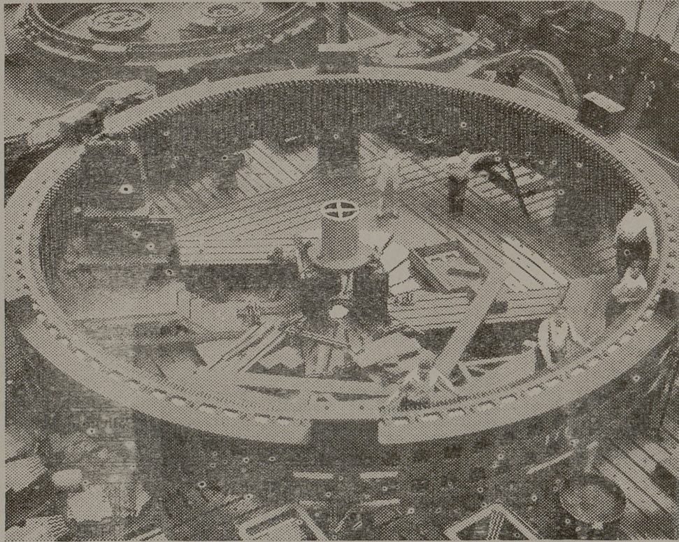
The picture above shows workmen assembling one of the huge Conowingo stators in the Westinghouse Works at East Pittsburgh. The men in the picture will give an idea of the tremendous size of these generators.
