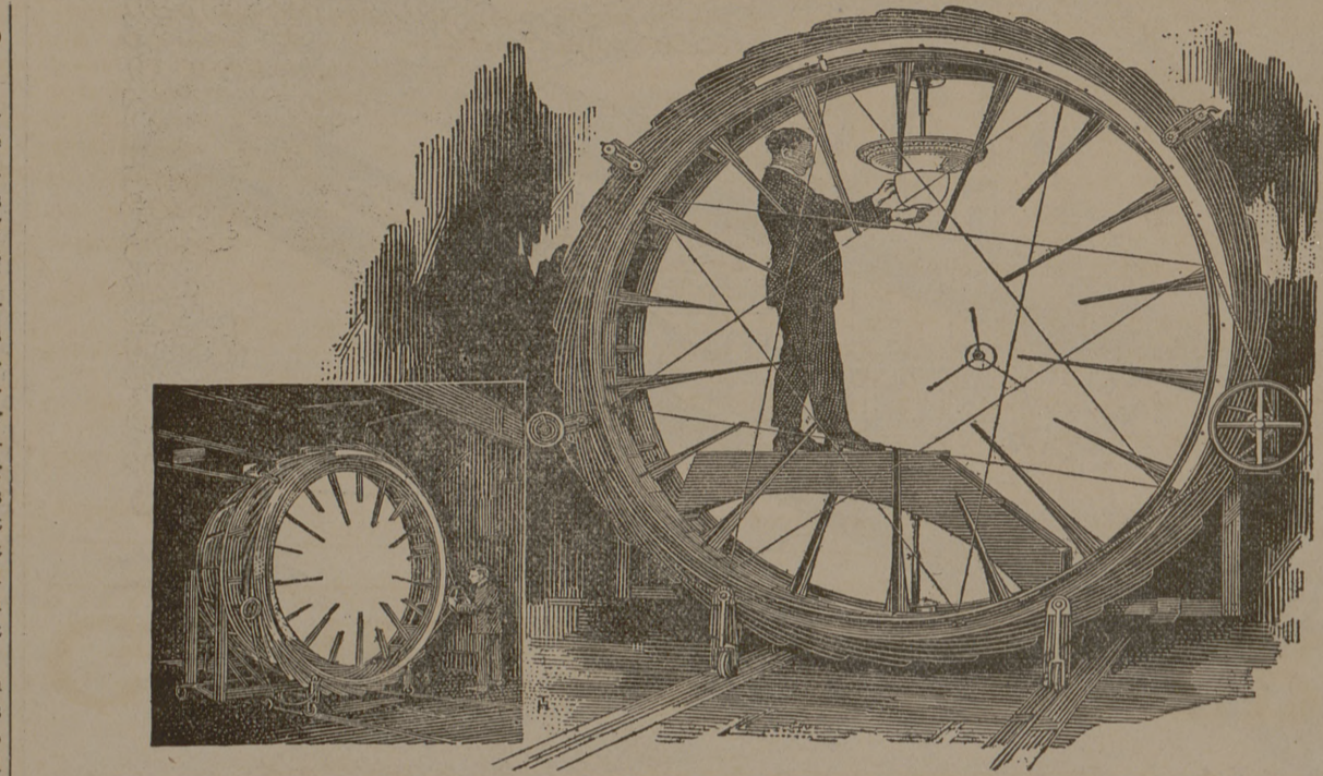
With the hemispherical integrator the illuminating engineer measures light intensities and distribution. These laboratory findings are practically applied to improve our everyday illumination.
